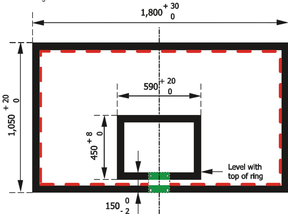
Diagram 2 Backboard markings
