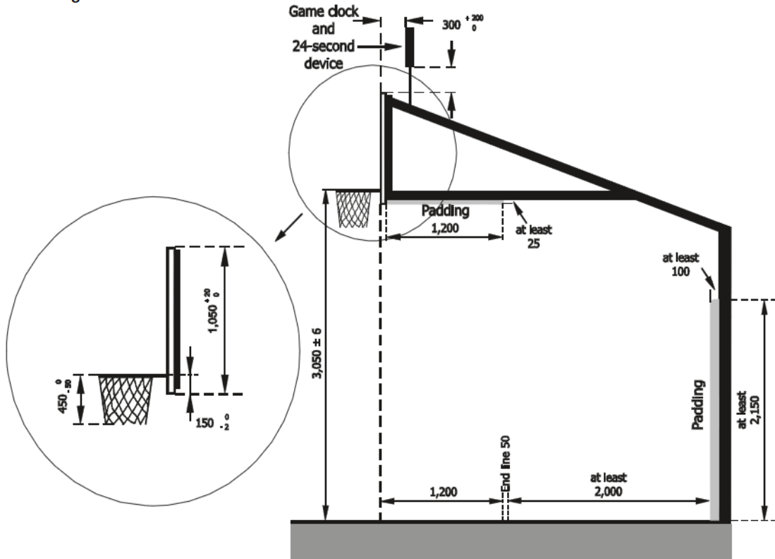
Diagram 1 Backstop unit
